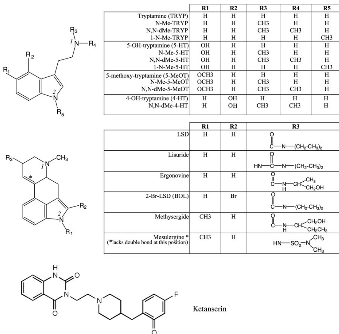
Fig. 1. Structures of ketanserine, unsubstituted and substituted tryptamines and ergolines. 1, amine nitrogen interacting with Ser3.36 and Asp3.32; 2, N1 nitrogen interacting with Ser5.46
