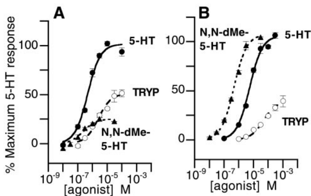
Fig. 2. Stimulation of accumulation of [ ^3 H]IP in (A) WT and (B) Ser3.36Ala mutant cell lines normalized with fit E_{\max} value for 5-HT equal to 100%, mean \pm S.E. of triplicate determinations. In this representative experiment, the values for WT and mutant were, respectively, 539 and 301 dpm for basal and 4245 and 6195 dpm for 5-HT E_{\max} .
